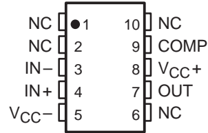
LM107 . . . U FLAT PACKAGE (TOP VIEW)
