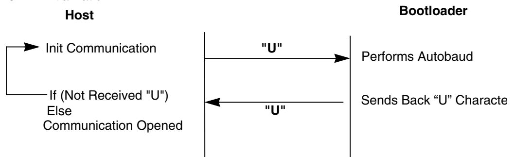
Figure 23-11. Initialization
