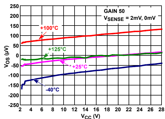
FIGURE 24. V_{OS} vs V_{CC} , V_{RS+} = 12V
