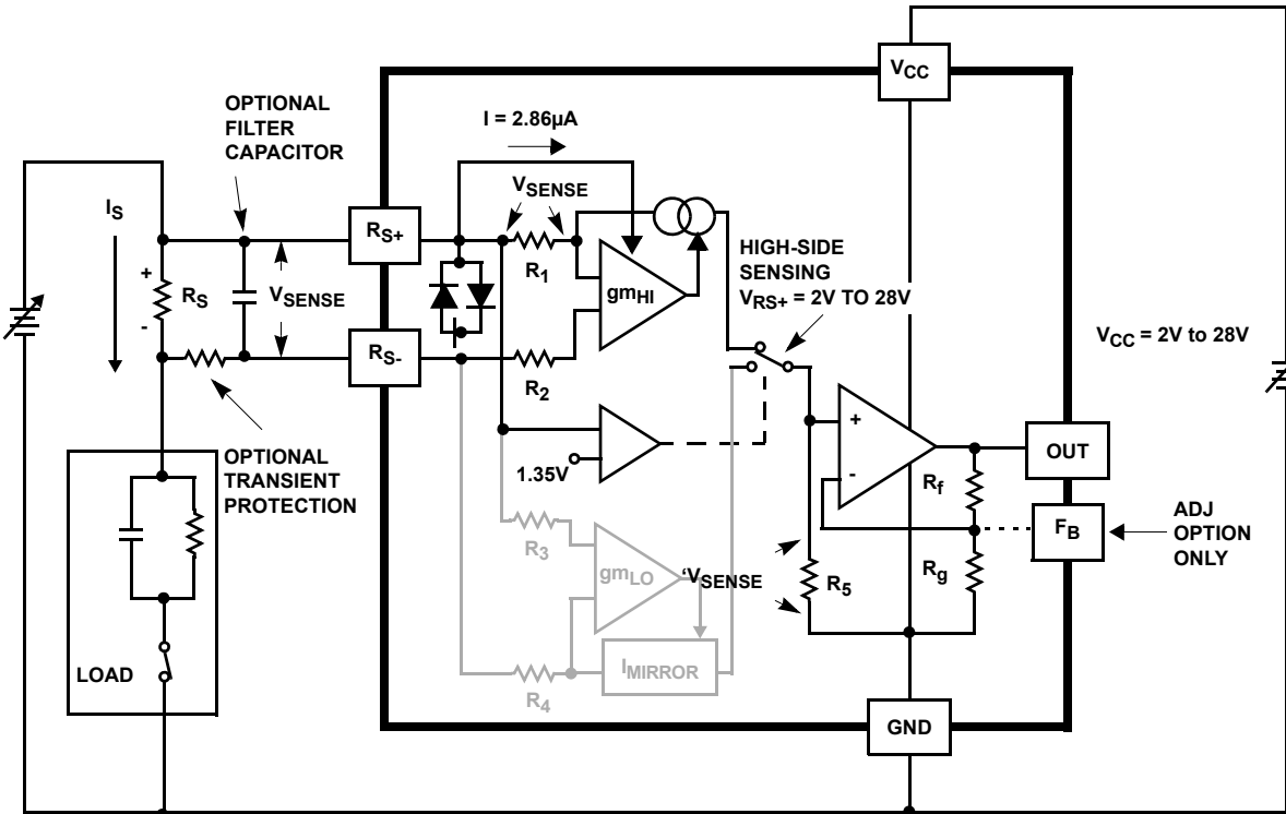
FIGURE 68. HIGH-SIDE CURRENT DETECTION
