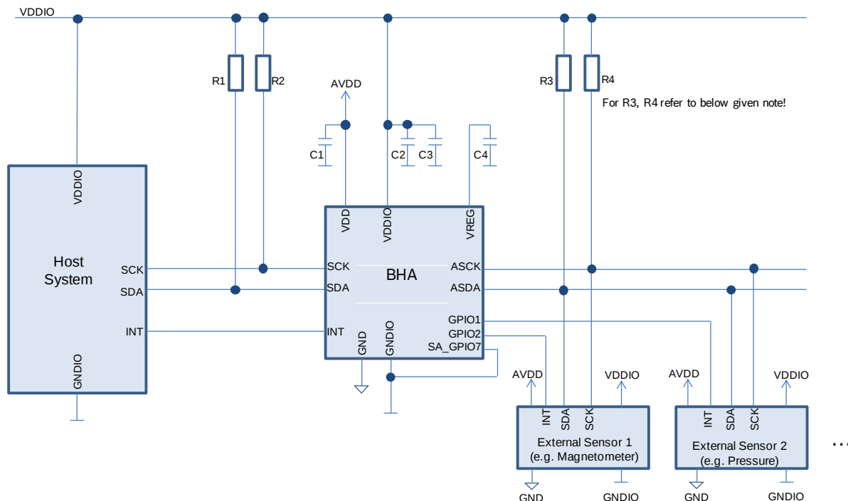
Figure 2: Reference Diagram
