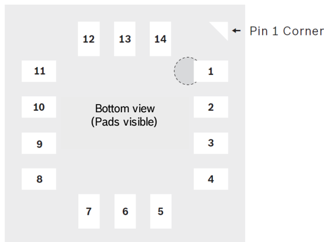
Figure 1: Pin Connections
