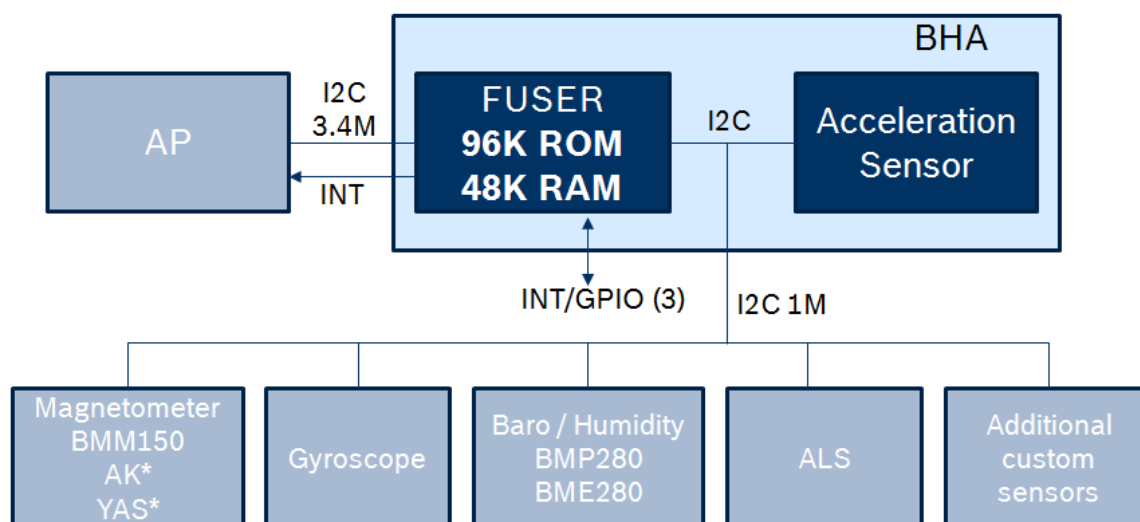
Figure 3: Block Diagram
