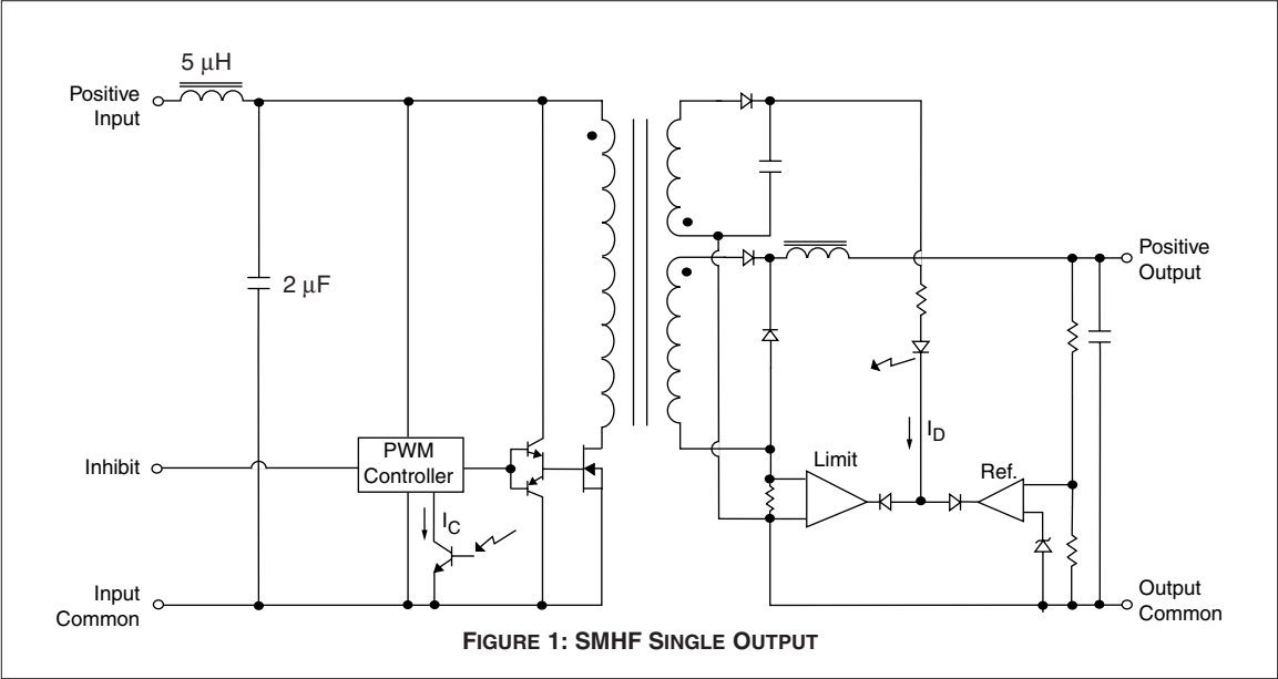
BLOCK DIAGRAM
