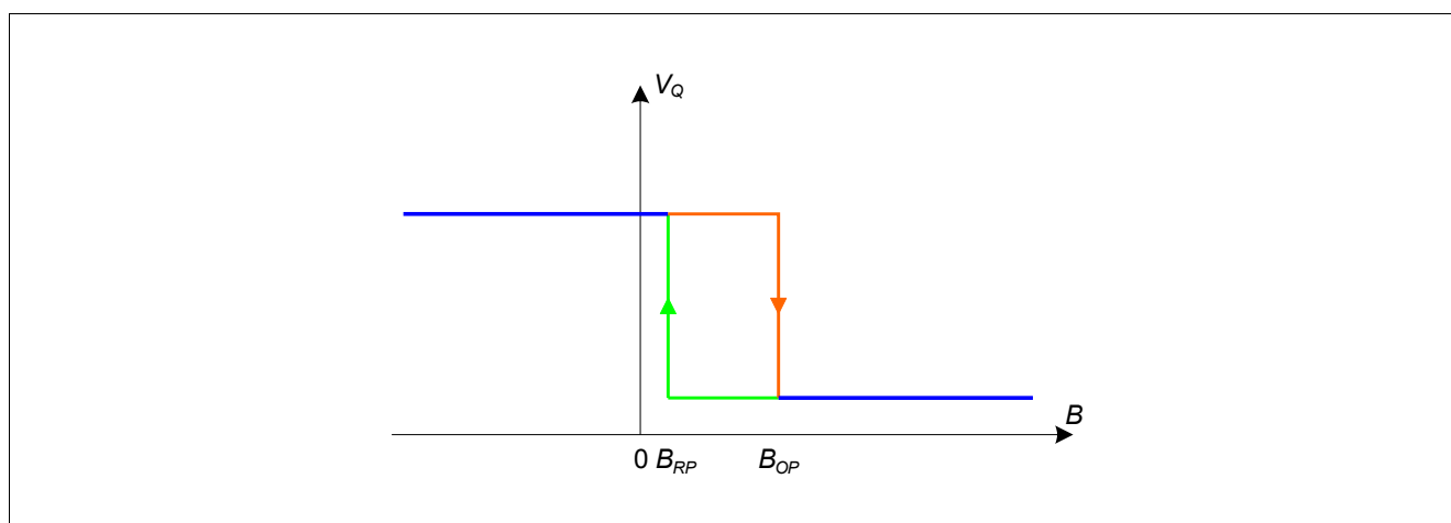
Figure 2-4 Output Signal TLE4964-5M
