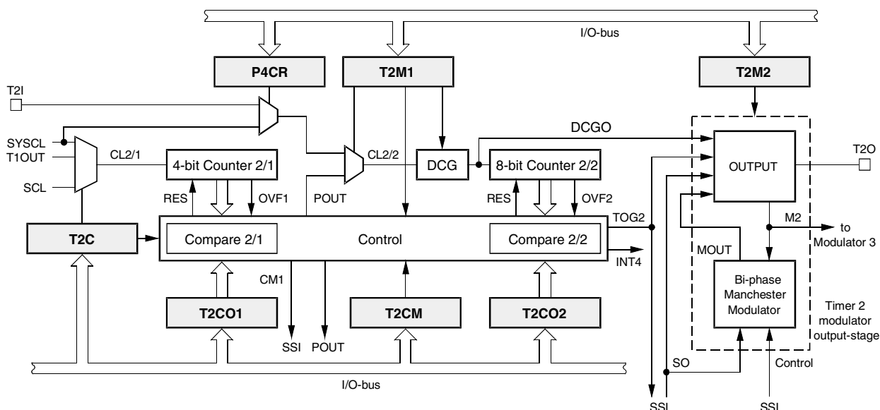
Figure 29. Timer 2
