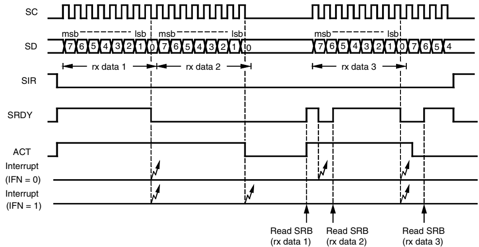
Figure 46. Example of 8-bit Synchronous Receive Operation
