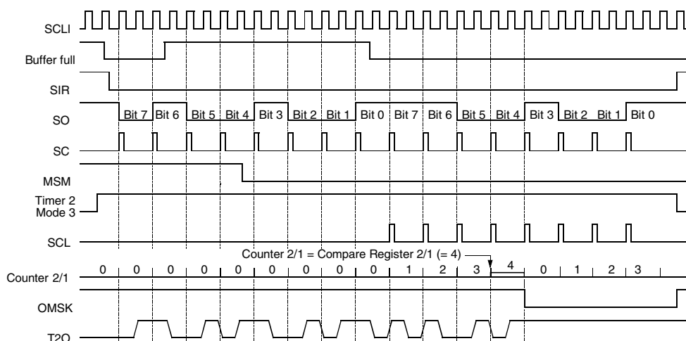
Figure 56. Manchester Modulation 2
