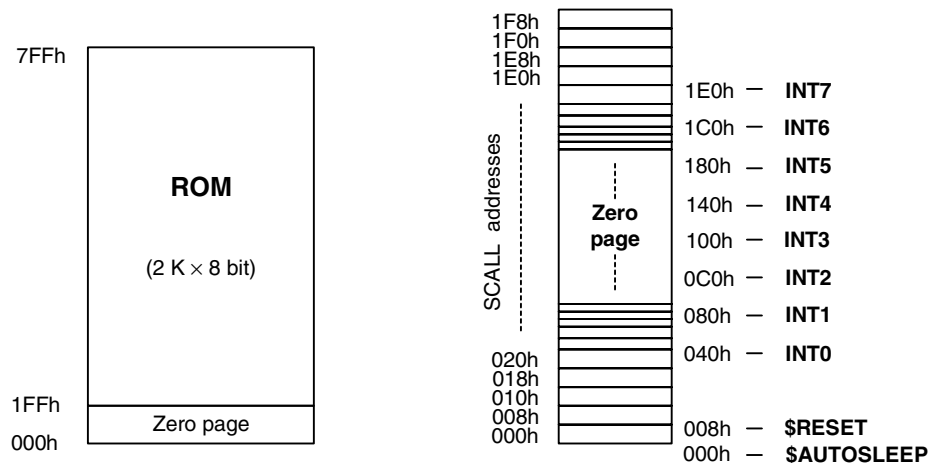
Figure 4. ROM Map
