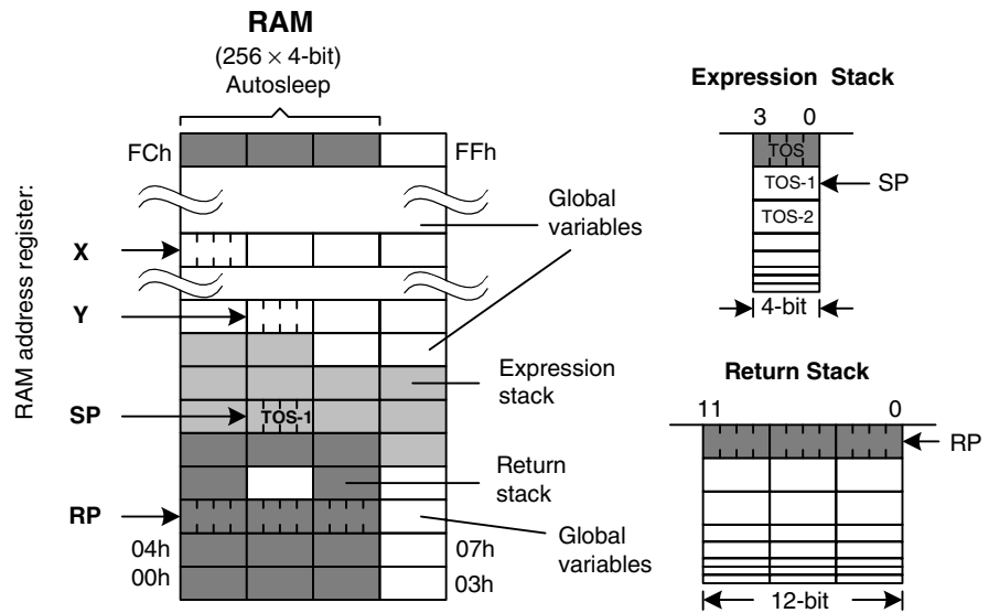
Figure 5. RAM Map
