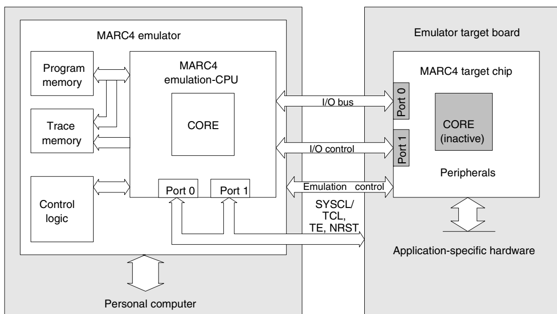
Figure 78. MARC4 Emulation
