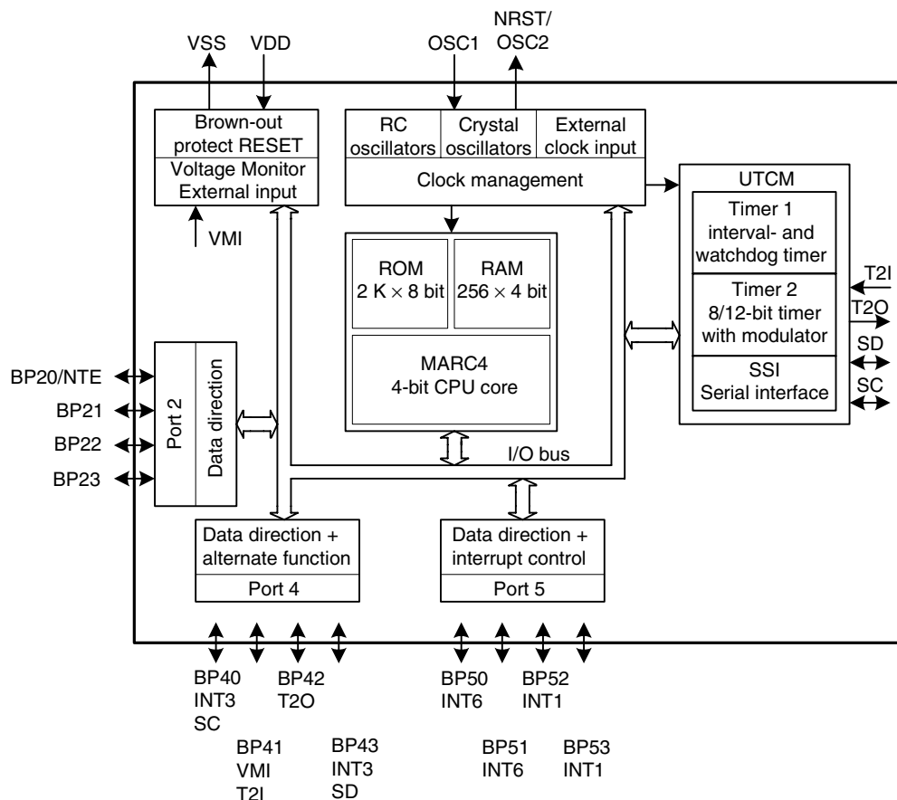
Figure 1. Block Diagram
