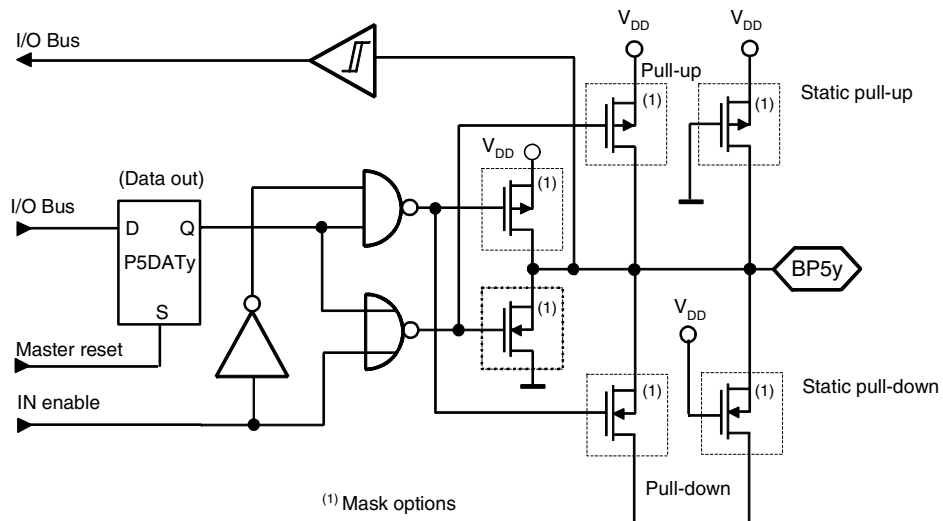
Figure 23. Bi-directional Port 5
