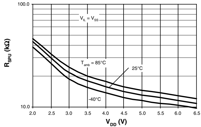
Figure 71. Strong Pull-up Resistor versus V_{DD}
