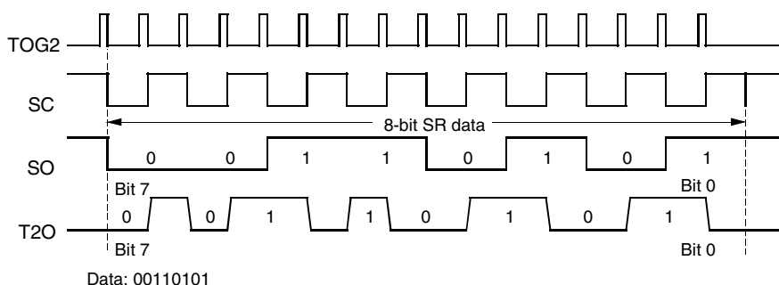
Figure 55. Manchester Modulation 1
