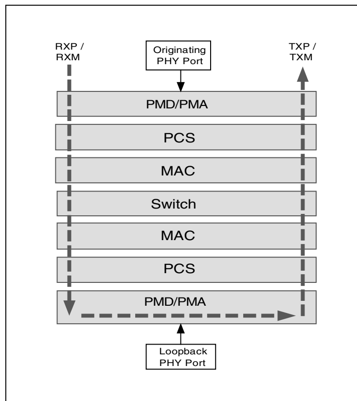
Figure 12. Loopback Path
