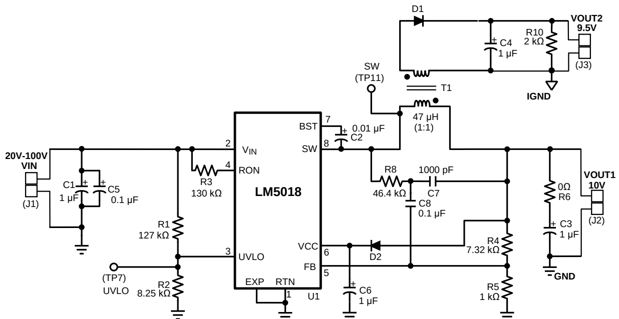
Figure 2. Complete Evaluation Board Schematic
