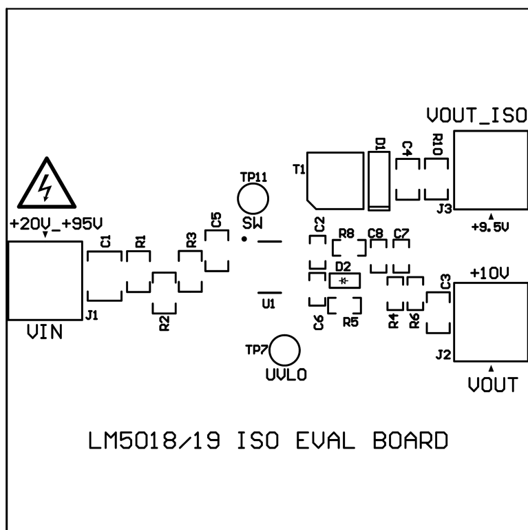
Figure 6. Board Silkscreen
