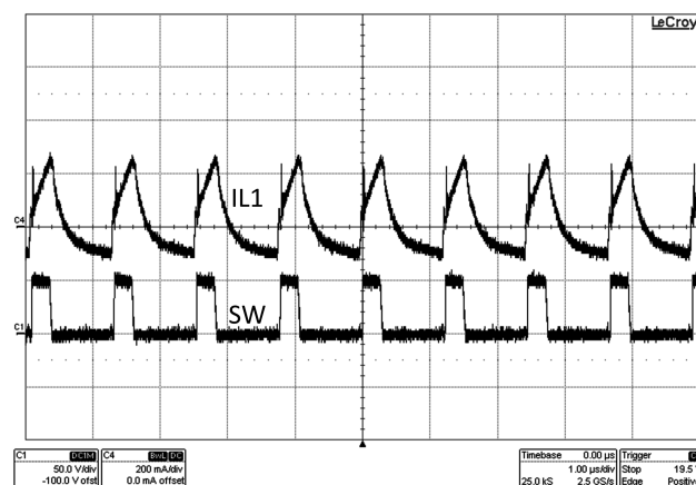
Figure 4. Steady State Waveform (VIN = 48V, IOUT1 = 0mA, IOUT2 = 100mA)
