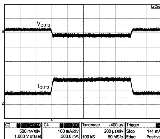
Figure 5. Step Load Response (VIN = 48V, IOUT1 = 0, Step Load on IOUT2 = 80mA to 180mA)
