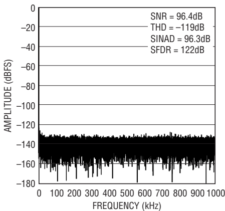
32k Point FFT f_S = 2\text{Mps} , f_{IN} = 2\text{kHz}
