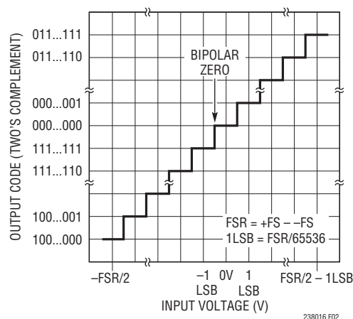
Figure 2. LTC2380-16 Transfer Function
