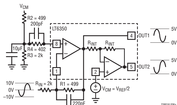
Figure 6a. LT6350 Converting a \pm 10\text{V} Single-Ended Signal to a \pm 5\text{V} Differential Input Signal
