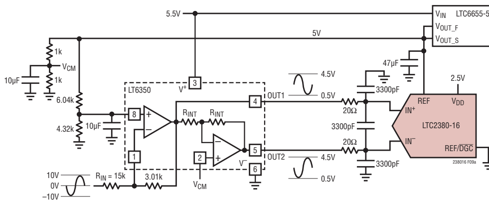
Figure 9a. LT6350 Configured to Accept a \pm 10\text{V} Input Signal While Running Off of a Single 5.5V Supply When Digital Gain Compression Is Enabled in the LTC2380-16
