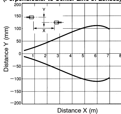
F3S-A482P (20-mm beam spacing)
