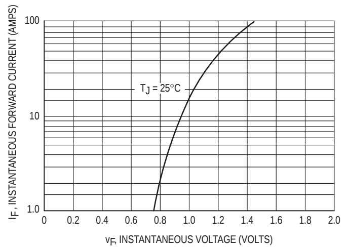
Figure 6. Typical Forward Voltage
