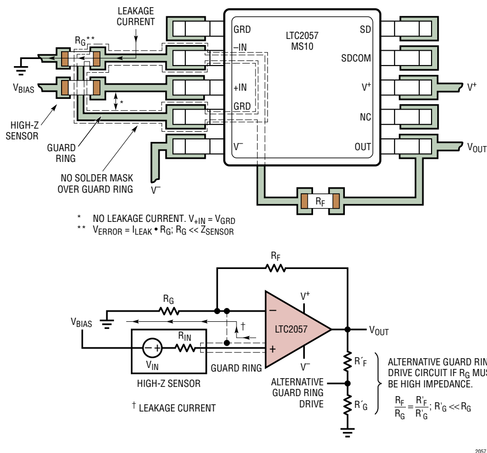
Figure 7a. Example Layout of Non-Inverting Amplifier with Leakage Guard Ring
