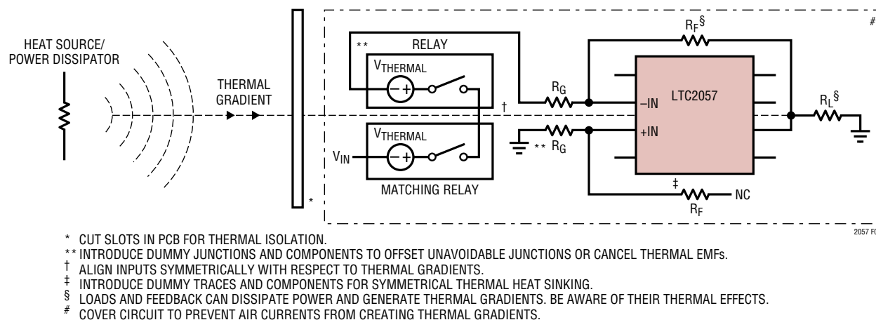
Figure 6. Techniques for Minimizing Thermocouple-Induced Errors
