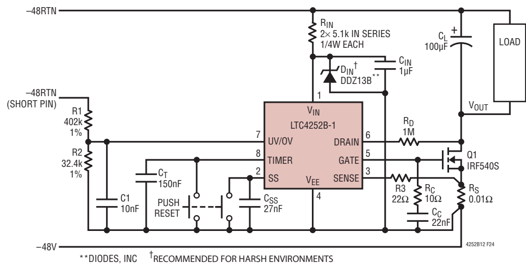
Figure 24. -48V/5A Application
