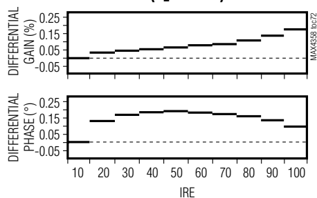
DIFFERENTIAL GAIN AND PHASE ( R_L = 150\Omega )
