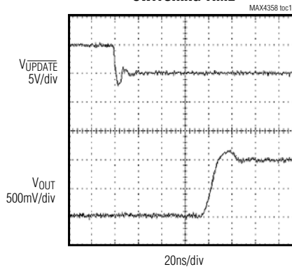
SWITCHING TIME
