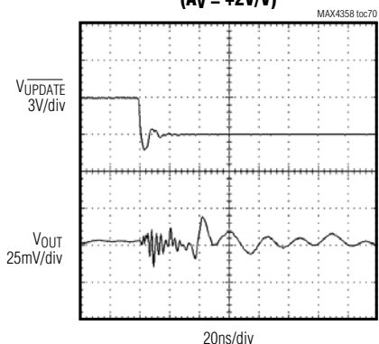
SWITCHING TRANSIENT GLITCH ( A_V = +2V/V )
