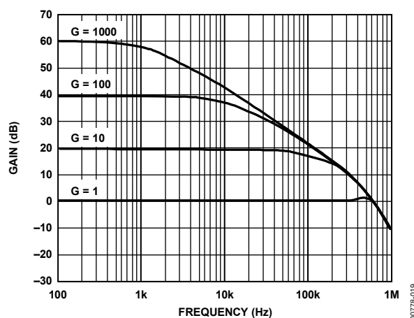
Figure 19. Gain vs. Frequency ( V_S = 5V , V_{REF} = 2.5V )
