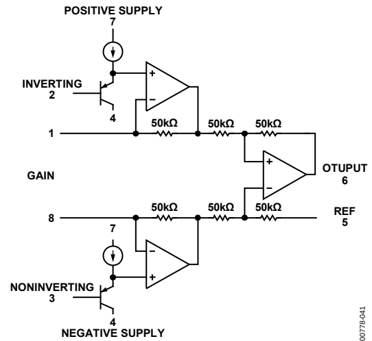
Figure 41. Simplified Schematic
