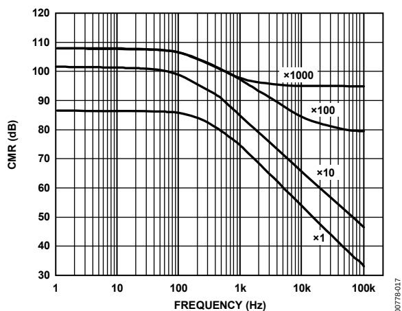
Figure 17. CMR vs. Frequency, V_S = 5V , V_{REF} = 2.5V
