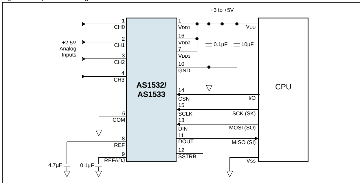
Figure 33. Operational Diagram
