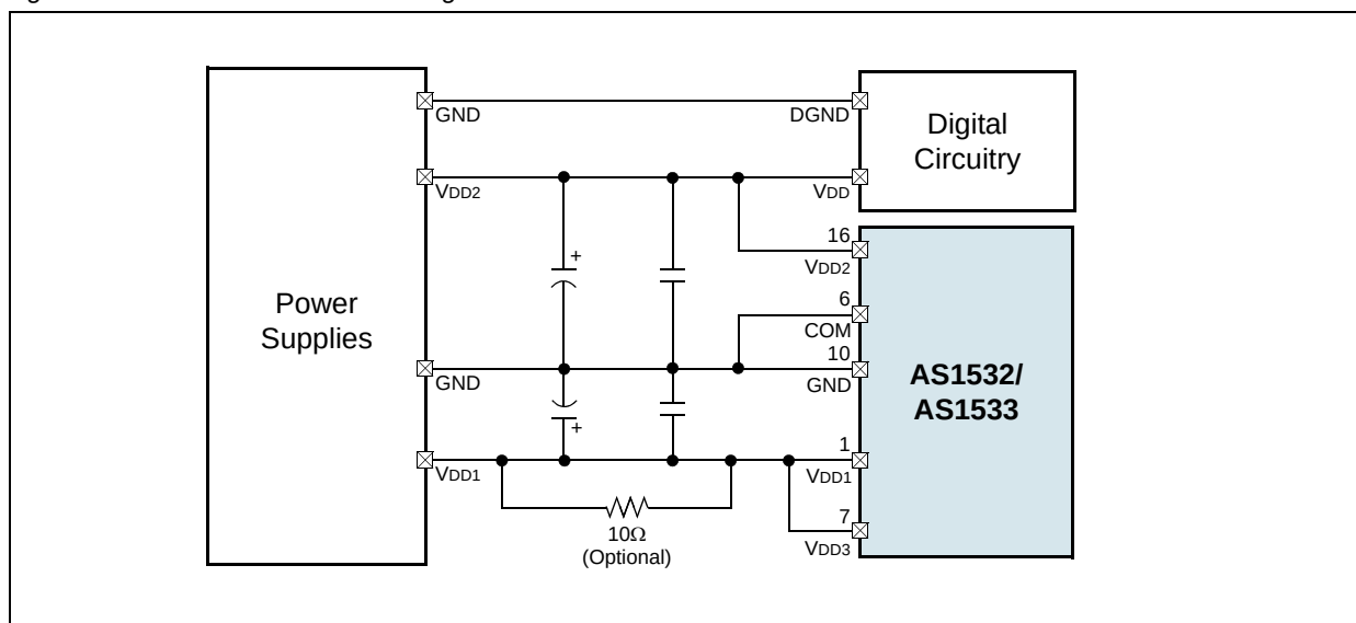
Figure 35. Recommended GND Design
