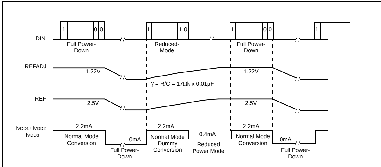
Figure 30. Full Power-Down Timing Waveforms (AS1533)
