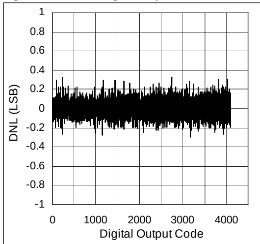
Figure 6. DNL vs. Digital Output Code
