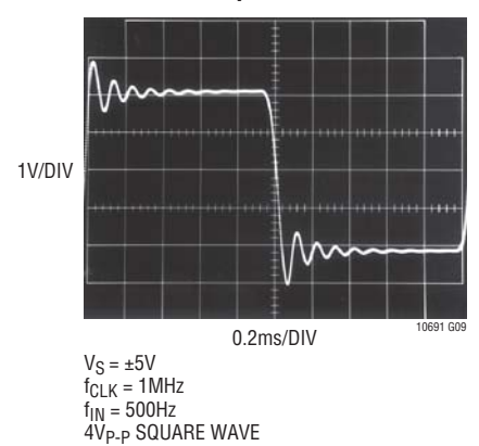
Transient Response
