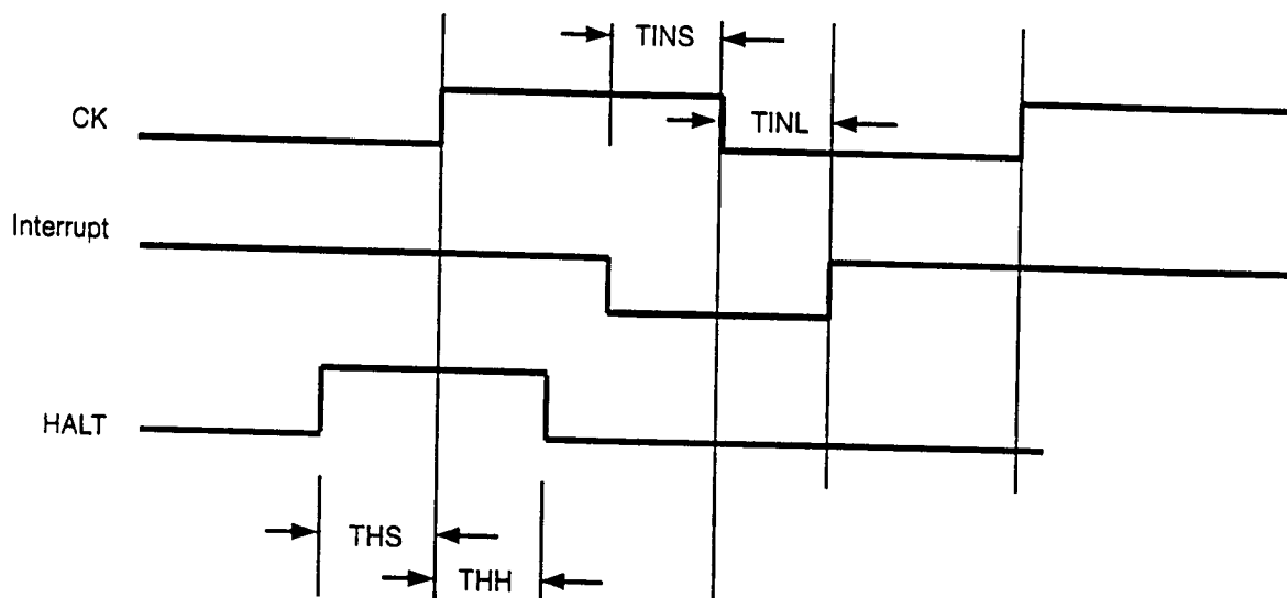
Figure 7. Interrupt/HALT Timing
