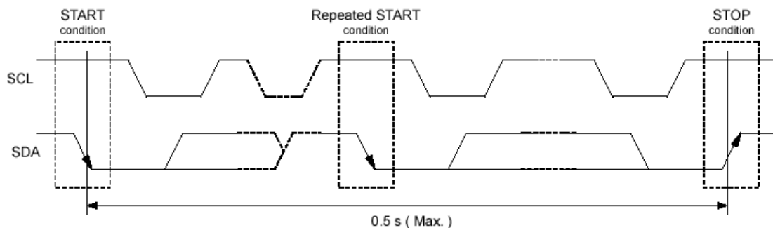
Fig3. Starting and stopping on I 2 C bus
