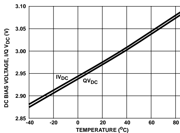
FIGURE 10. DC BIAS VOLTAGE ( I/Q V_{DC} ) vs TEMPERATURE
