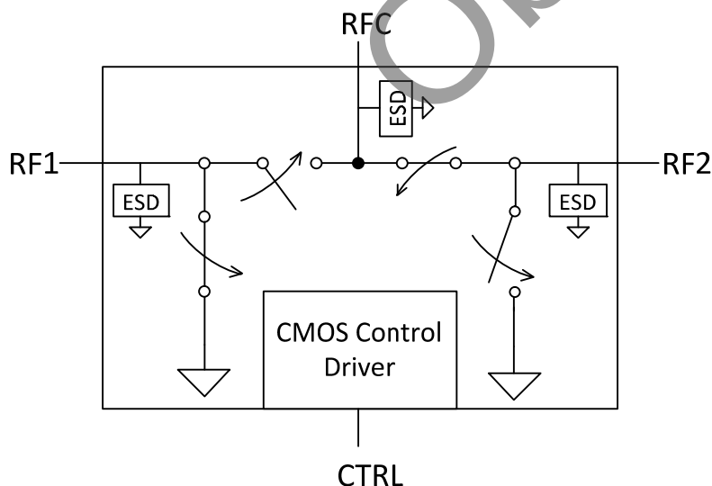
Figure 1. Functional Diagram
