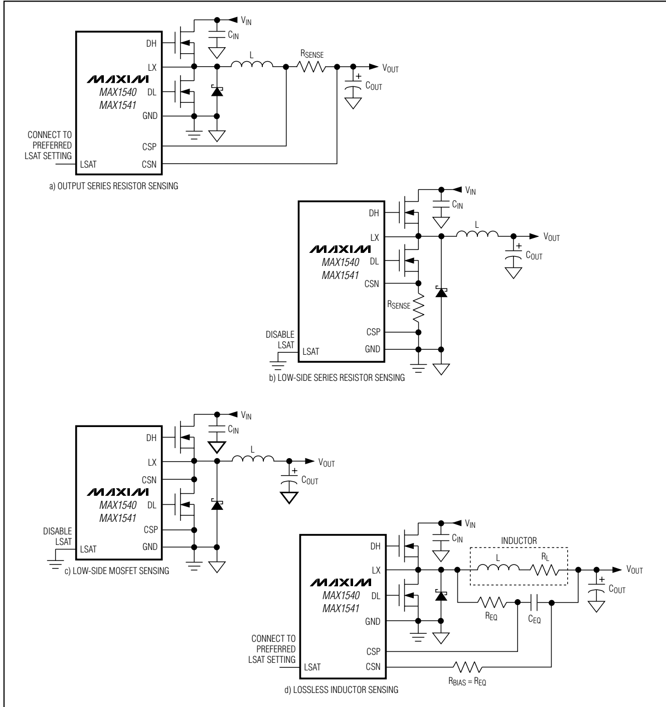
Figure 14. Current-Sense Configurations
