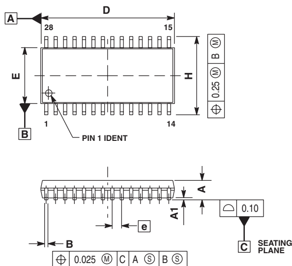
Figure 17. Outline Dimensions for SOG Package (Case Outline 751F-05, Issue F)
