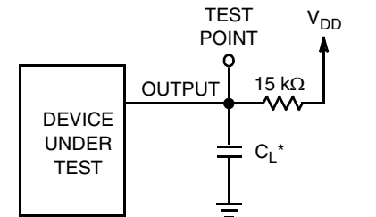
Figure 9c. Maximum Output Transition Time
