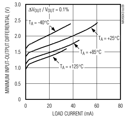
MINIMUM INPUT-OUTPUT DIFFERENTIAL vs. LOAD CURRENT ( V_{OUT} = 2.5V )
