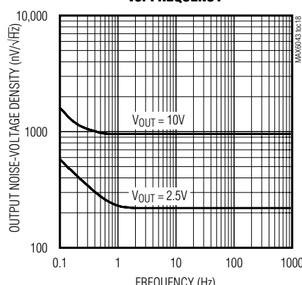
OUTPUT NOISE-VOLTAGE DENSITY vs. FREQUENCY
