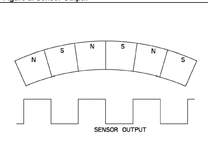
Figure 2. Sensor Output
