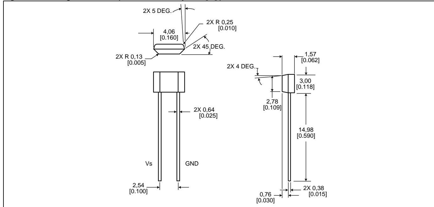
Figure 4. Mounting Dimensions (For reference only. mm/[in].)
