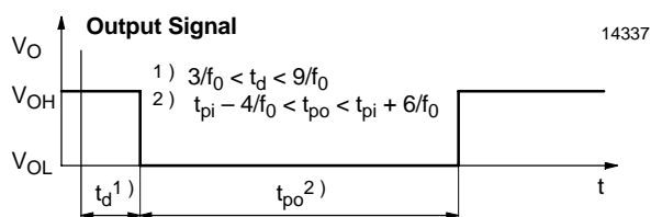
Figure 7. Output Function
