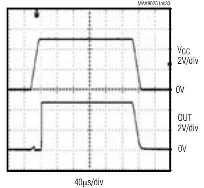
POWER-UP/POWER-DOWN RESPONSE
