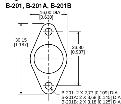
Figure 19. 3001/3004 Brackets
