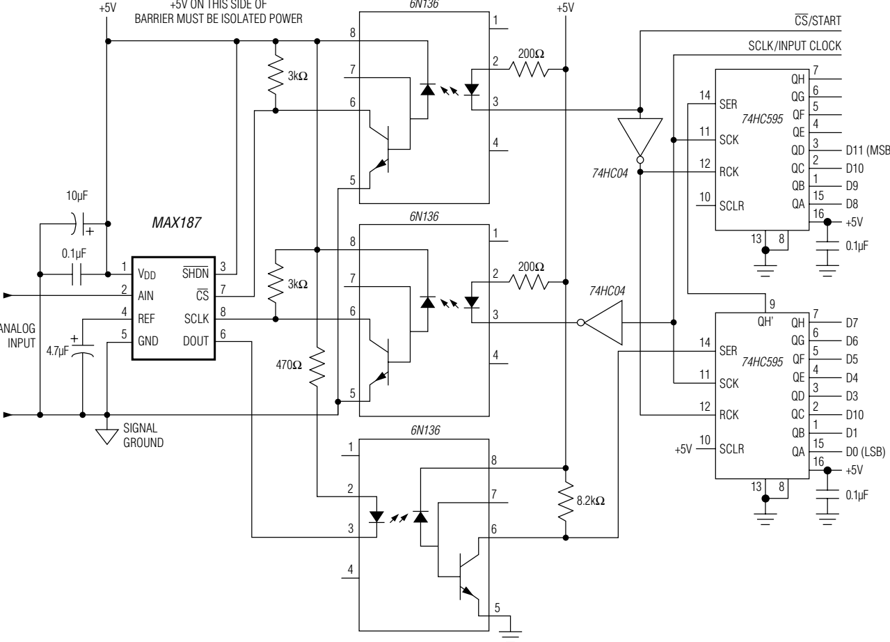
Figure 16. 12-Bit Isolated ADC
