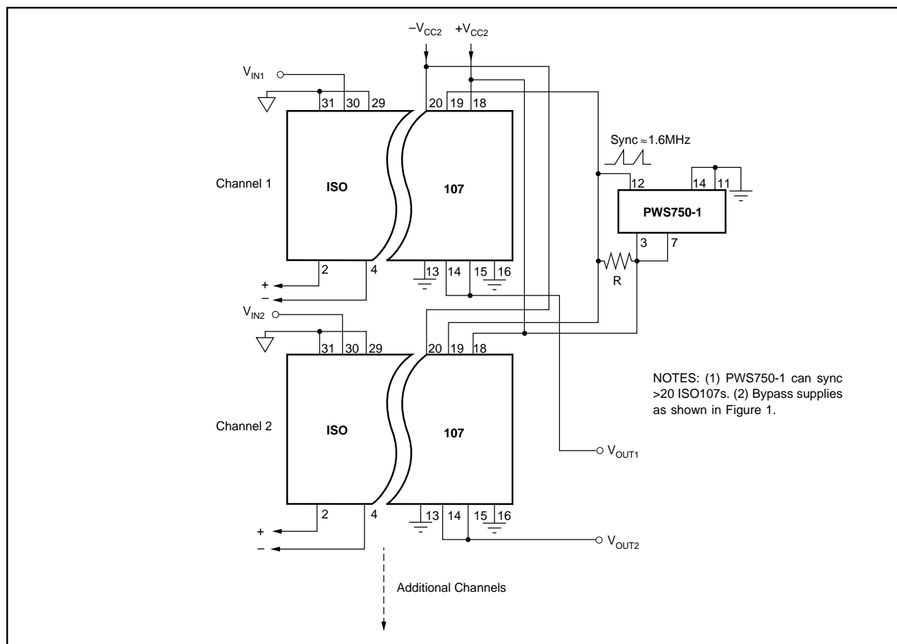
FIGURE 6. Synchronized-Multichannel Isolation.
