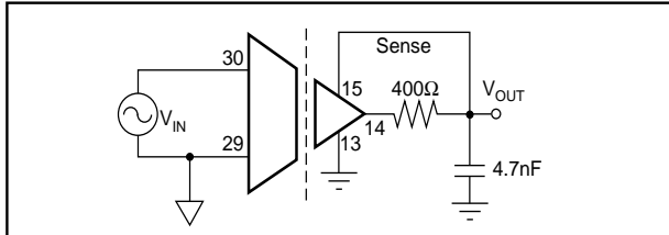
FIGURE 4. Ripple Reduction.
