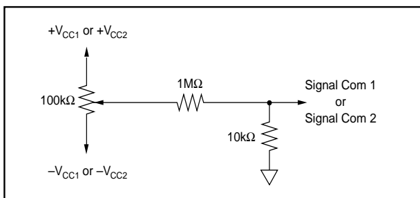
FIGURE 3. V_{OS} Adjust.
