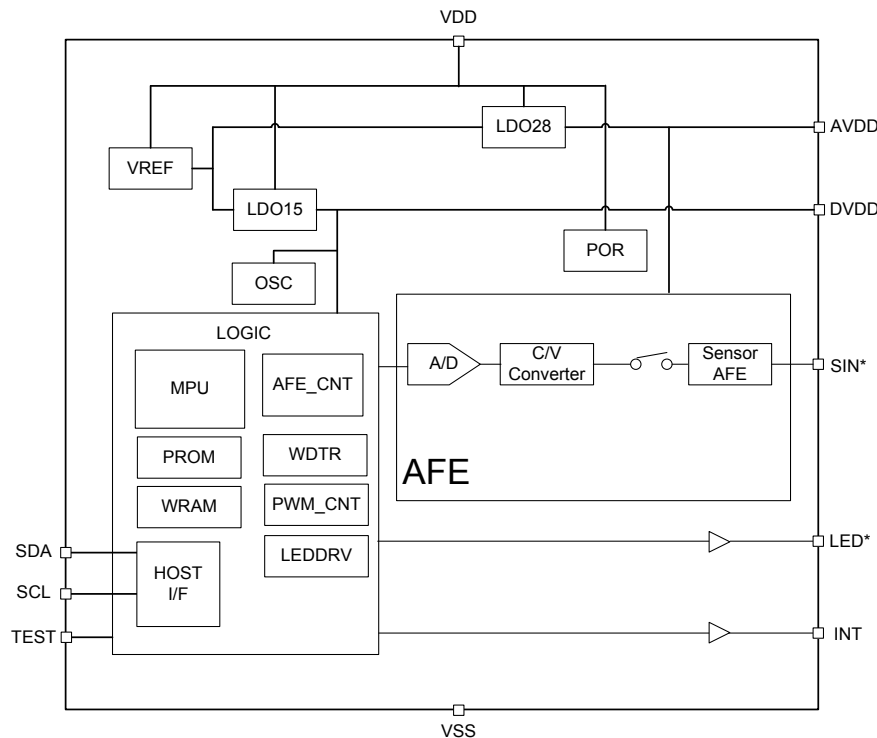
Figure 8. Block Diagram
