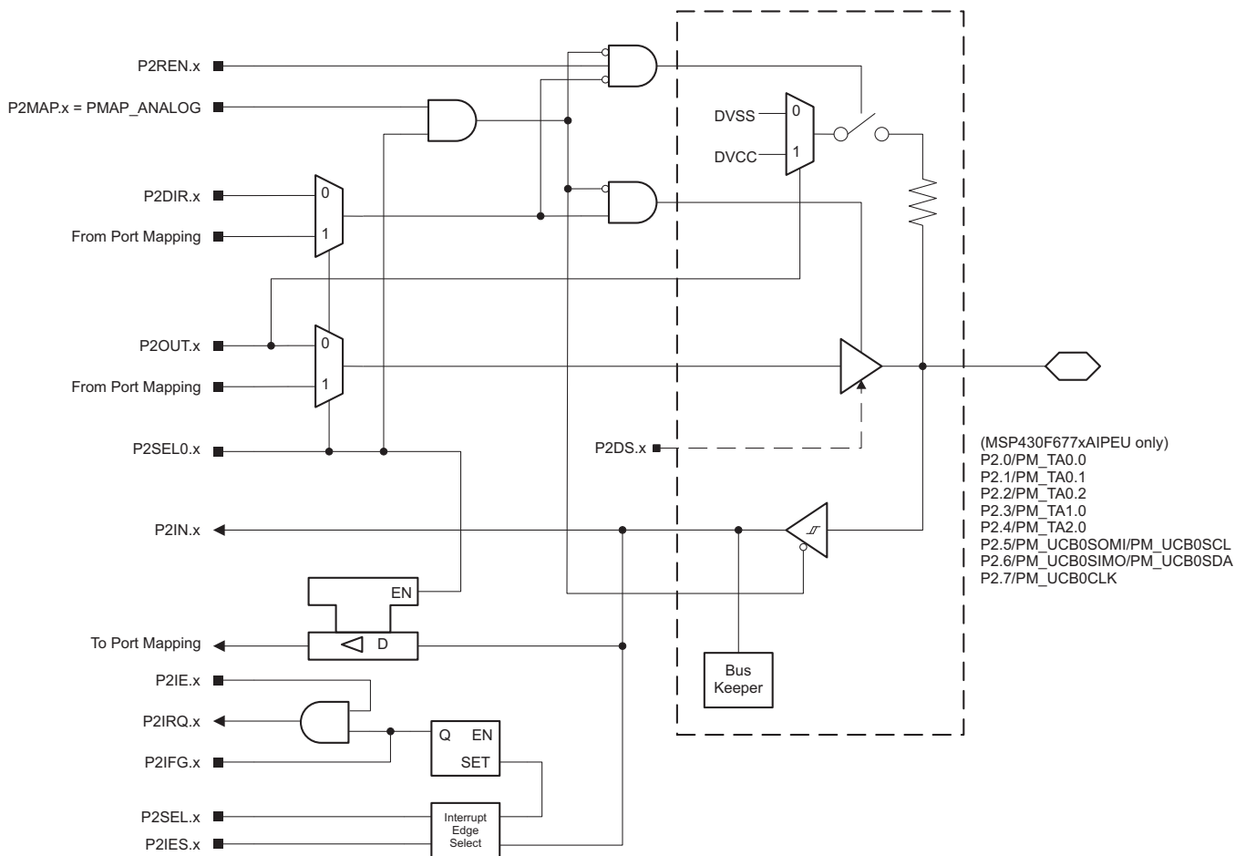
Figure 6-10. Port P2 (P2.0 to P2.7) Diagram (PEU Package Only)
