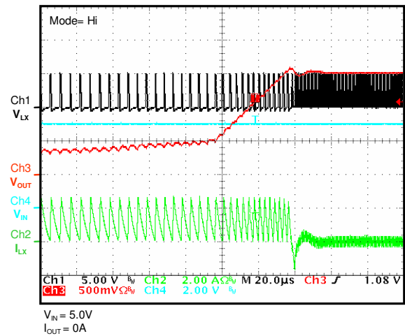
Recovery from OCP ( V_{OUT}=1.5V )
