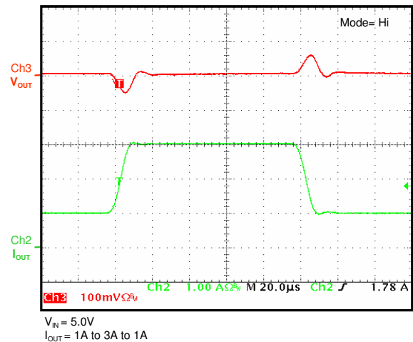
Transient Response ( V_{OUT}=3.3V , I_{STEP}=2A )
