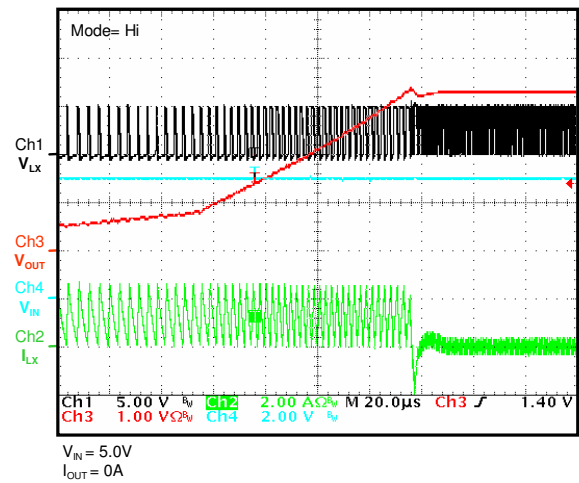
Recovery from OCP ( V_{OUT}=3.3V )
