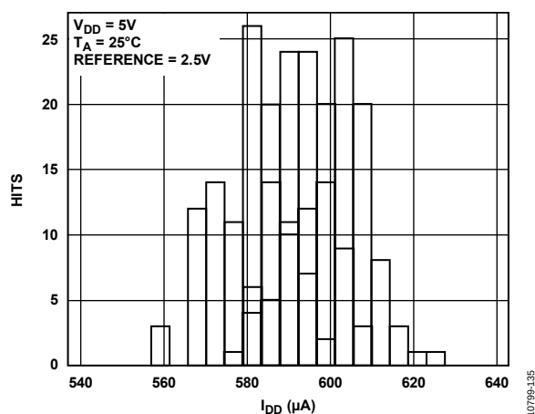
Figure 19. I_{DD} Histogram at 5 V
