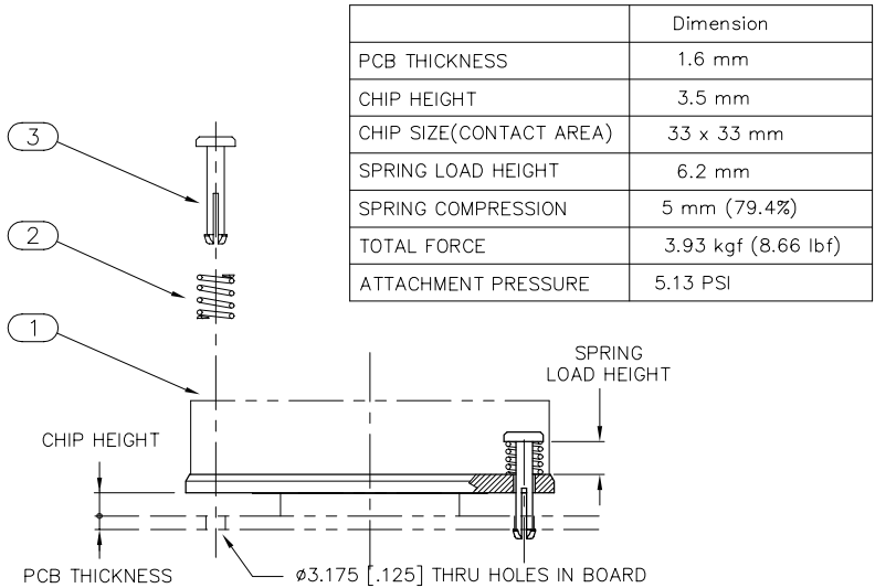
ASSEMBLY IMAGE (REFERENCE ONLY / DO NOT SCALE)
