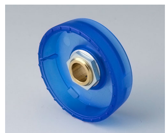
B8341086 STAR-KNOBS 41, with knurls PC (UL 94 HB) saphire 41x14mm 8mm
