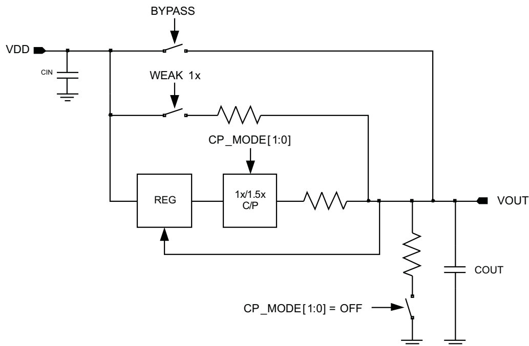
Figure 1. Functional Model of Charge Pump
