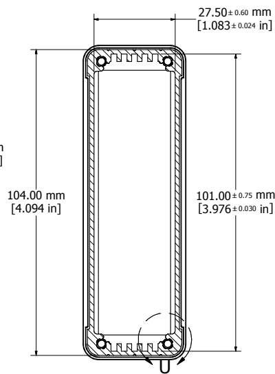
SECTION T-T
