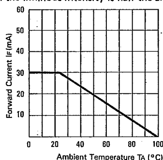
FIG. 43 FORWARD CURRENT DERATING CURVE
