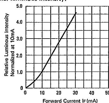
FIG. 44 RELATIVE LUMINOUS INTENSITY VS. FORWARD CURRENT
