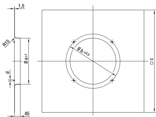
Square wall rings with short nozzle for S-Range axial fans
