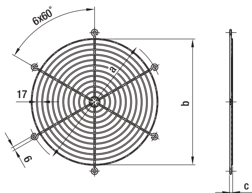
Guard grilles (e.g. for backward curved centrifugal fans)
