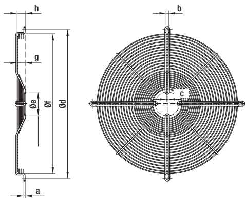
Guard grilles for S-Range axial fans
