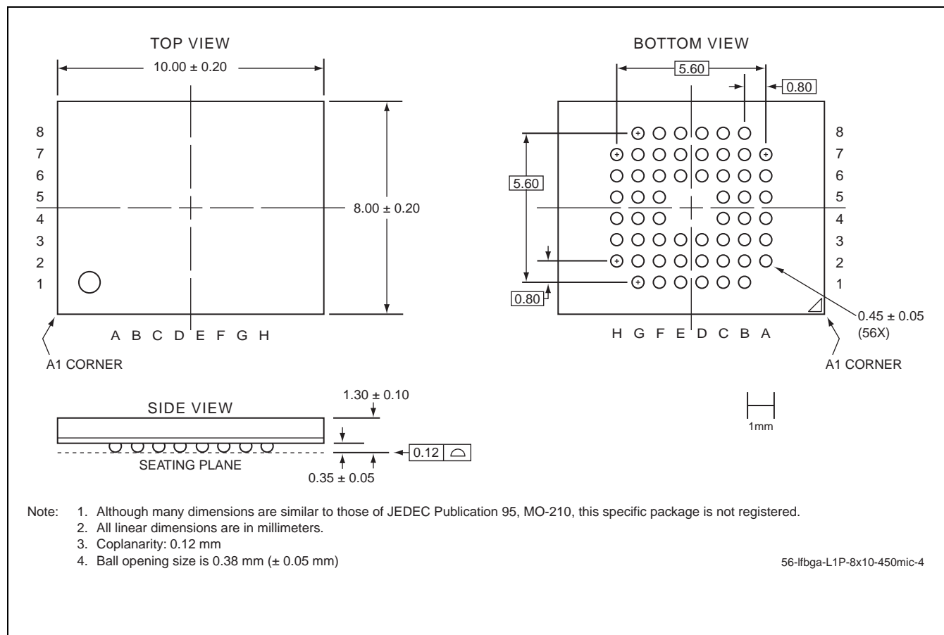
FIGURE 27: 56-ball Low-profile, Fine-pitch Ball Grid Array (LFBGA) 8mm x 10mm Greenliant Package Code: L1P
