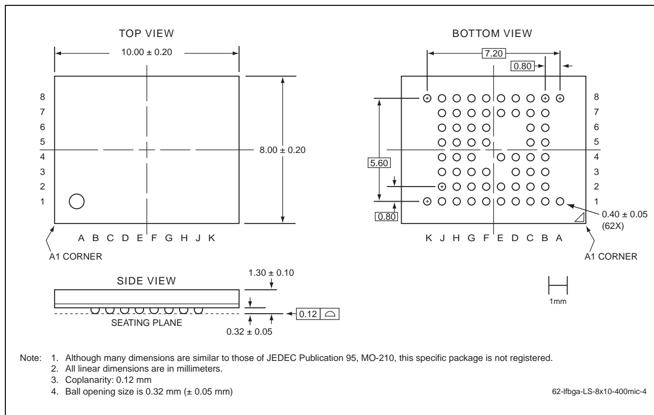
FIGURE 28: 62-ball Low-profile, Fine-pitch Ball Grid Array (LFBGA) 8mm x 10mm Greenliant Package Code: LS
