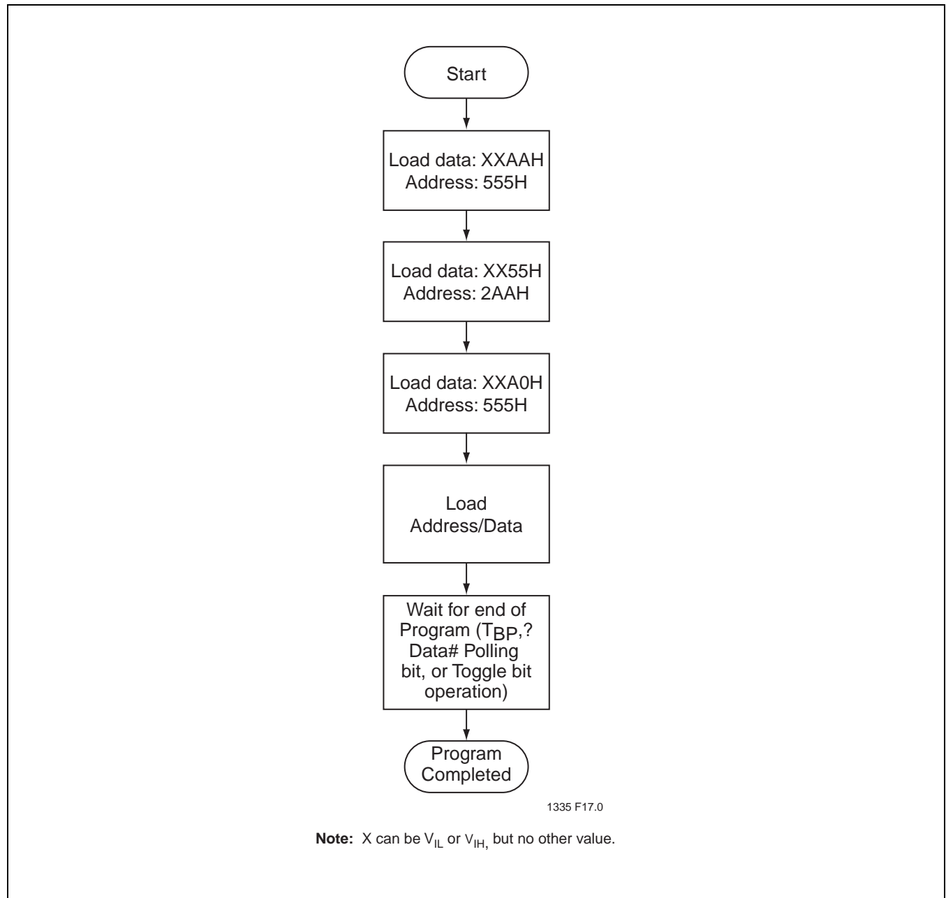
FIGURE 22: Program Algorithm
