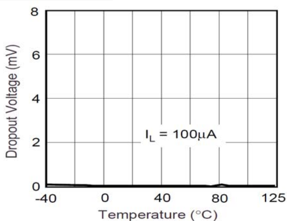
Figure 19. Dropout Voltage
