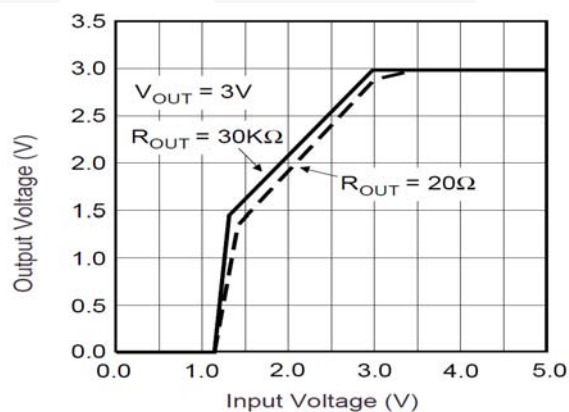
Figure 18. Dropout Characteristics
