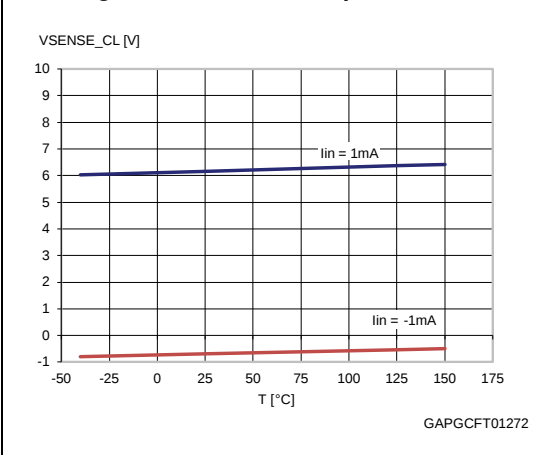
Figure 33: Vsense clamp vs. Tcase
