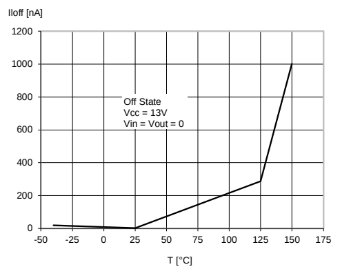
Figure 15: OFF-state output current
