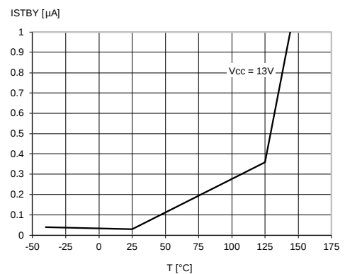
Figure 16: Standby current
