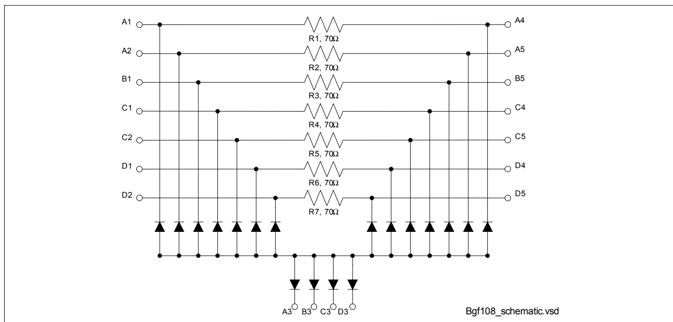
Figure 1 Schematic
