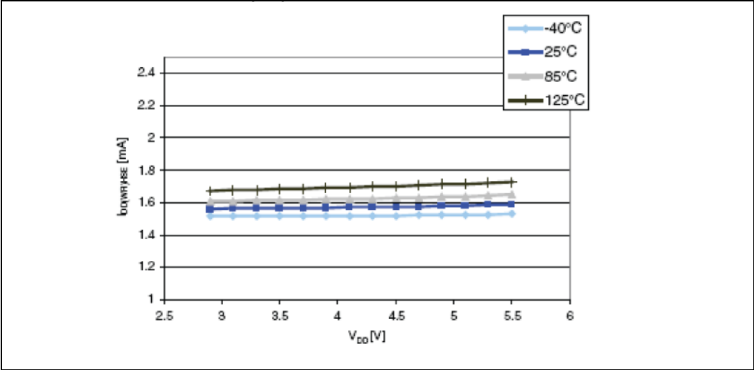
Figure 16. Typ I_{DD(WFI)} vs. V_{DD} HSE external clock, f_{CPU} = 16 MHz
