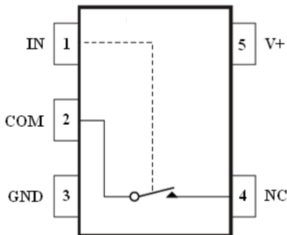
PI3A125B SOT23-5/SC70-5 Package (Top View)
