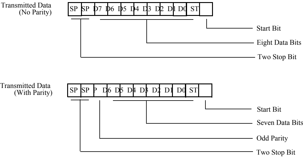
Figure 9-9. Transmitter Data Formats
