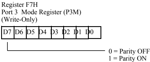
Figure 9-8. Port 3 Mode Register (P3M) Parity
