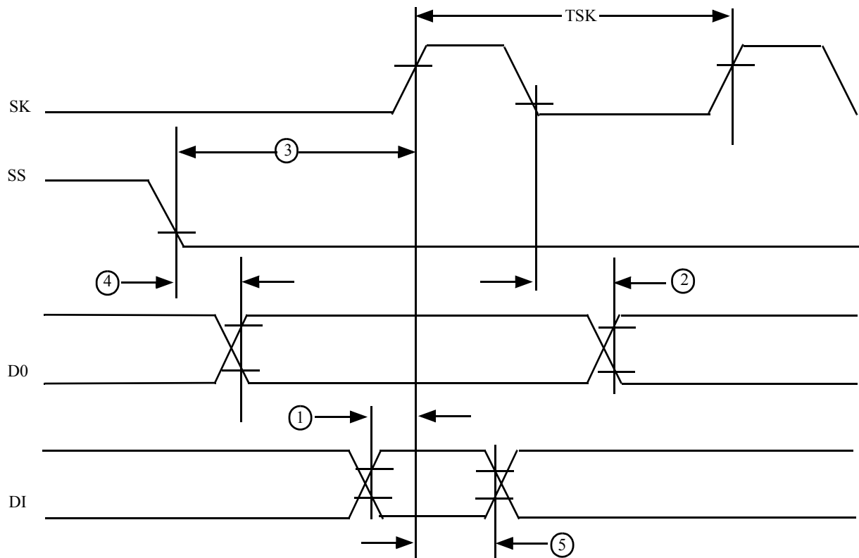
Figure 9-14. SPI Timing
