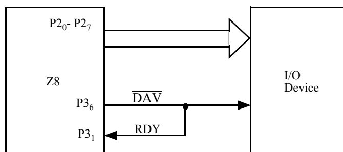
Figure 5-25. Output Strobed Handshake on Port 2
