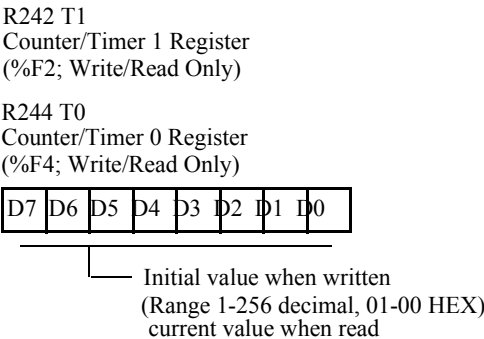
Figure 6-5. Counter / Timer 0 and 1 Registers
