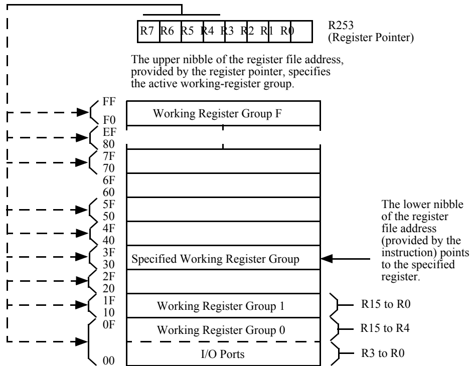
Figure 2-4. Register Pointer
