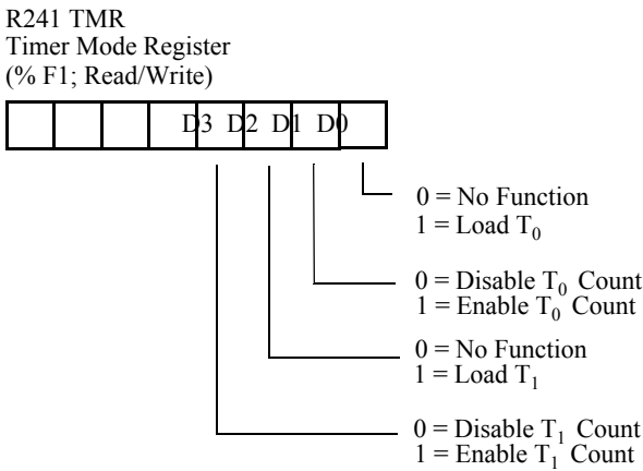
Figure 6-6. Timer Mode Register
