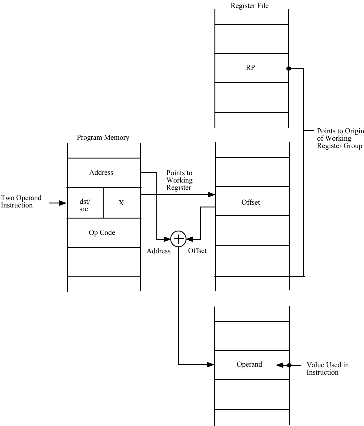
Figure 11-5. Indexed Register Addressing
