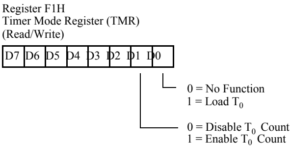
Figure 9-5. Timer Mode Register (TMR) Bit Rate Generation
