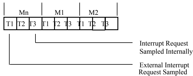
Figure 7-6. Interrupt Request Timing
