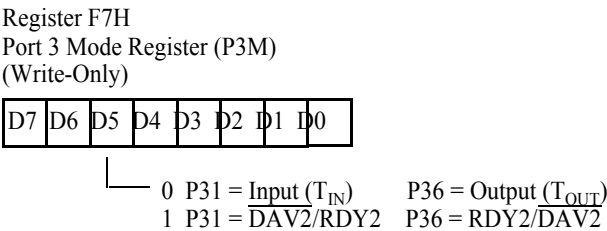
Figure 6-10. Port 3 Mode Register (T OUT Operation)
