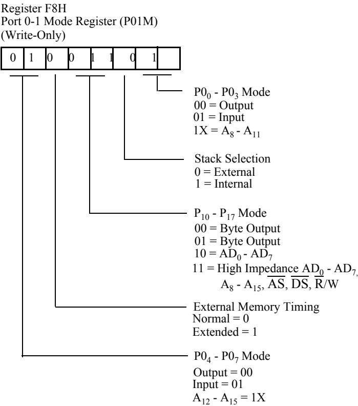
Figure 5-27. Port 0/1 Reset
