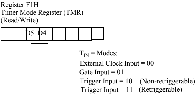
Figure 6-13. Timer Mode Register (T IN Operation)
