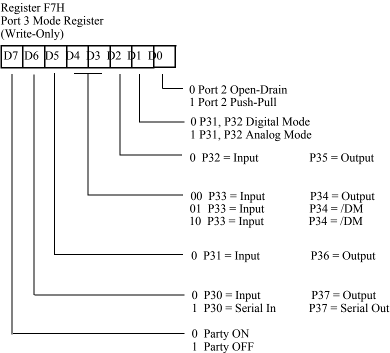
Figure 5-22. Port 3 Mode Register Configuration
