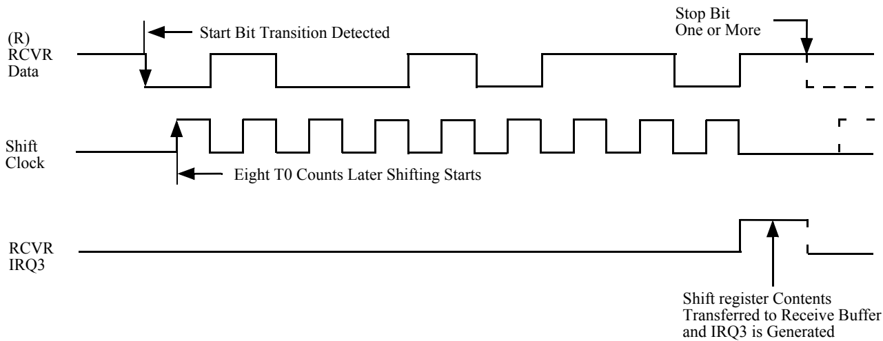
Figure 9-6. Receiver Timing
