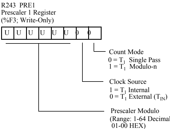
Figure 6-4. Prescaler 1 Register
