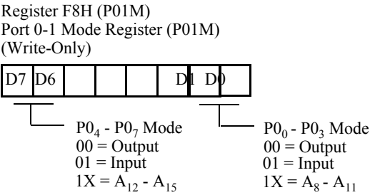
Figure 5-5. Port 0 I/O Operation
