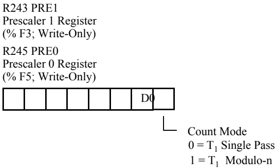
Figure 6-7. Starting The Count
