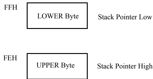
Figure 2-9. Stack Pointer
