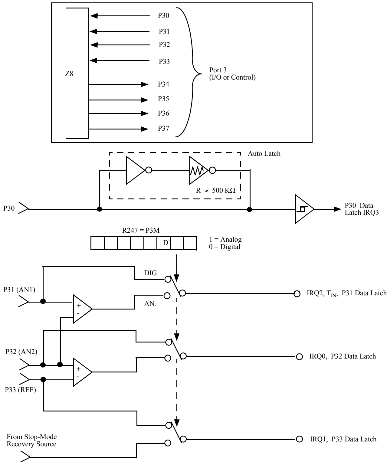
Figure 5-18. Port 3 Configuration with Comparator, Auto Latch, and Schmitt-Trigger
