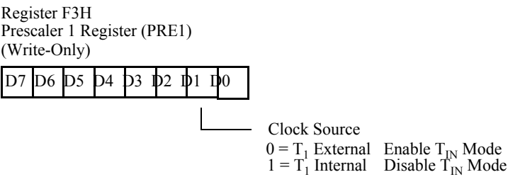
Figure 6-14. Prescaler 1 Register (T IN Operation)
