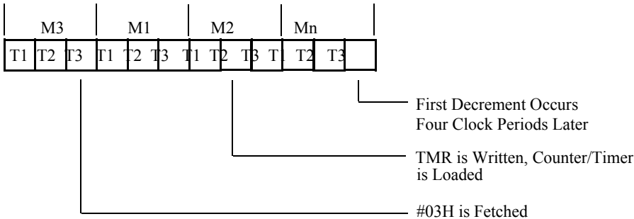
Figure 6-8. Counting Modes
