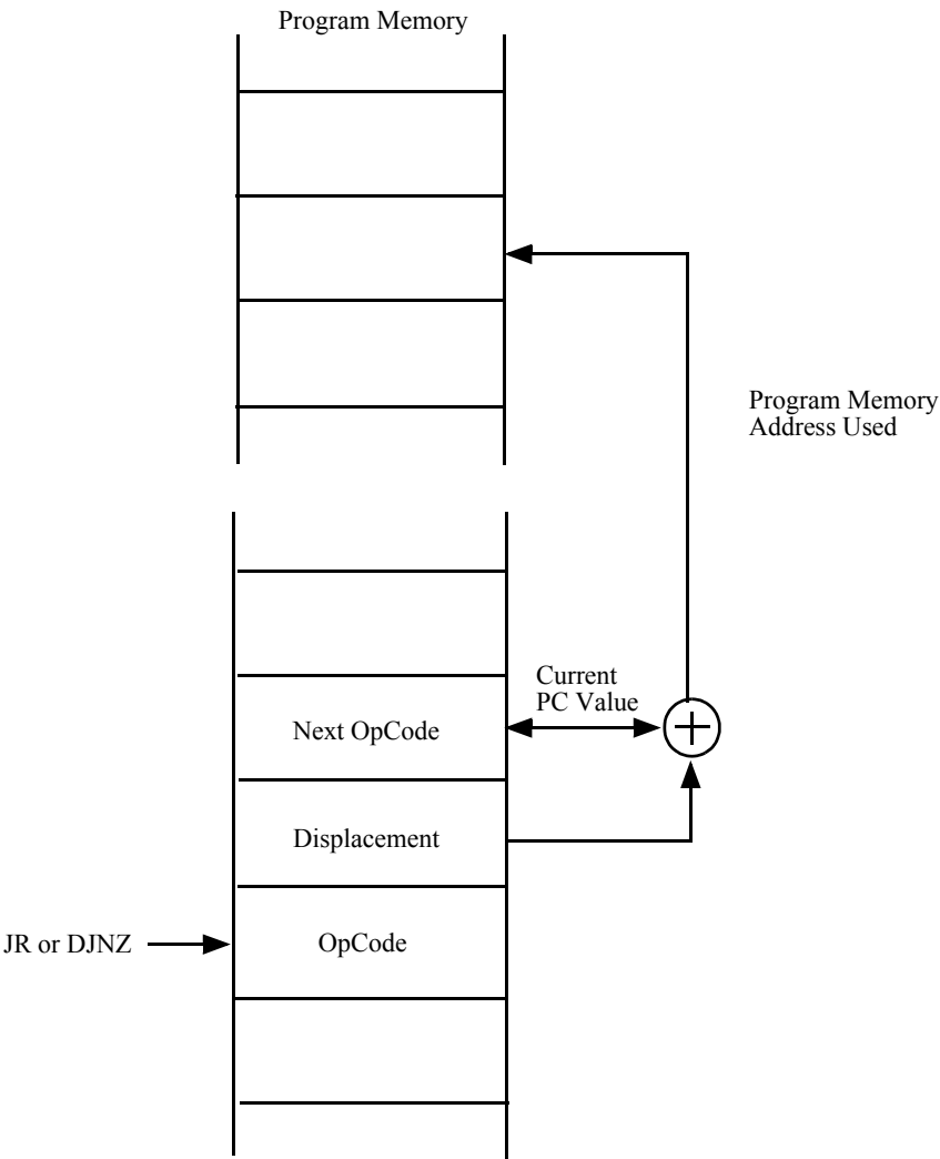
Figure 11-7. Relative Addressing
