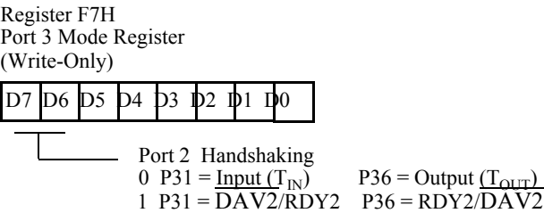
Figure 5-15. Port 2 Handshake Configuration
