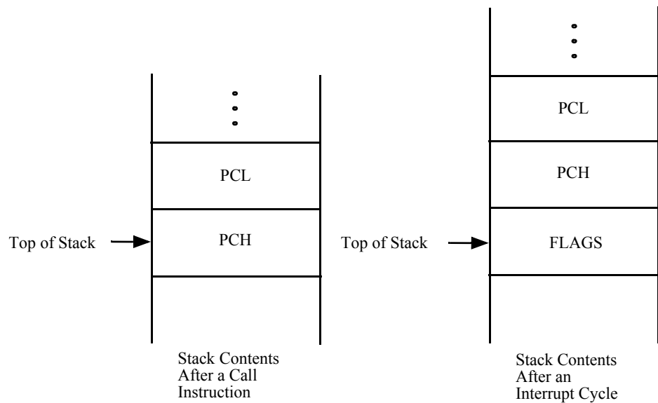
Figure 2-10. Stack Operations
