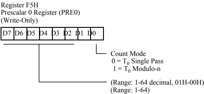
Figure 9-4. Prescaler 0 Register (PRE0) Bit-Rate Generation
