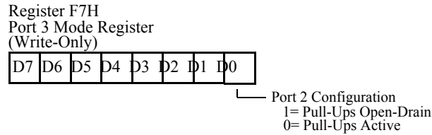
Figure 5-34. Port 2 Configuration
