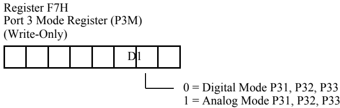
Figure 5-30. Port 3 Input Analog Selection
