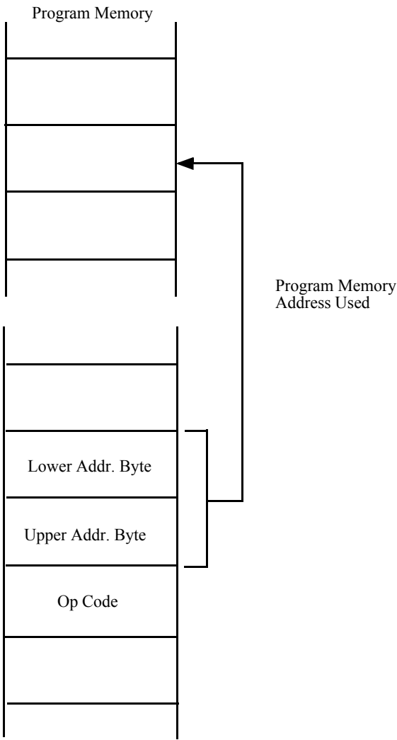
Figure 11-6. Direct Addressing
