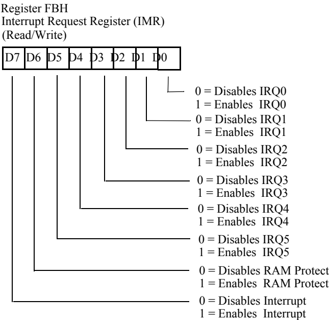
Figure 7-8. Interrupt Mask Register
