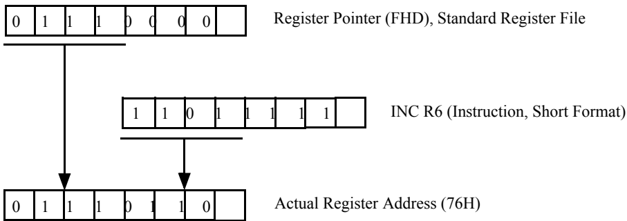
Figure 2-3. Working Register Addressing Examples
