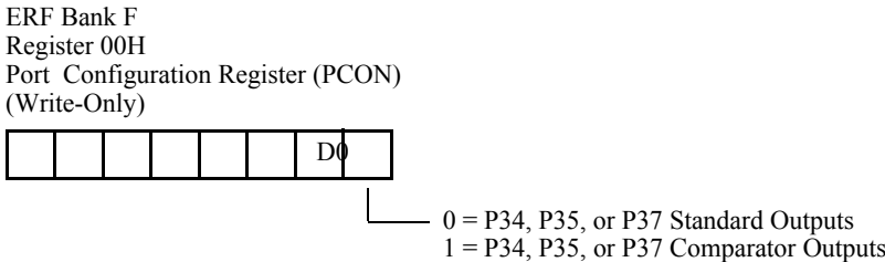
Figure 5-31. Port 3 Comparator Output Selection
