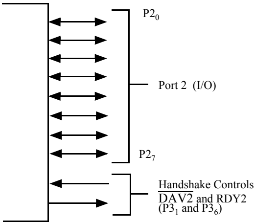
Figure 5-16. Port 2 Handshaking
