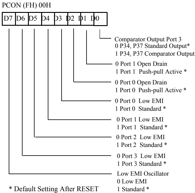
Figure 5-35. Port Configuration Register (PCON) (Write-Only)
