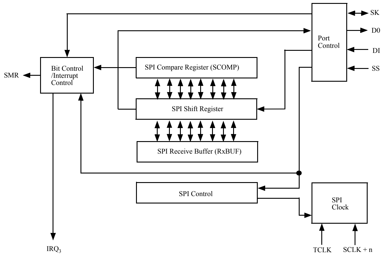
Figure 9-15. SPI Logic
