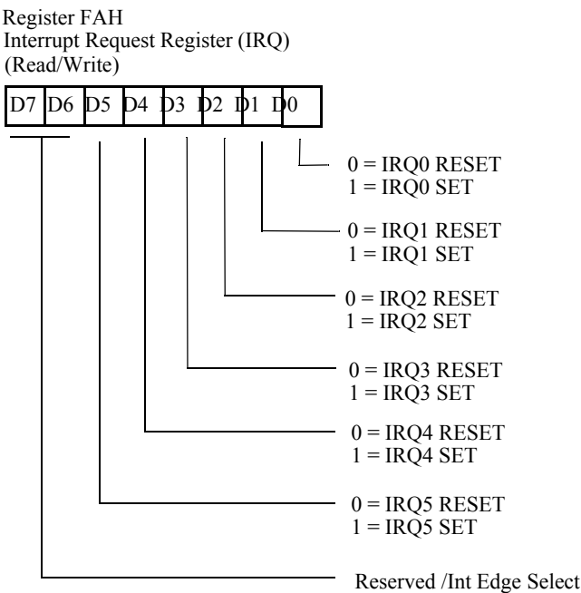
Figure 7-9. Interrupt Request Register
