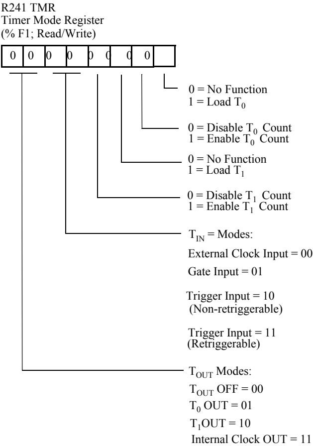
Figure 6-22. Timer Mode Register Reset
