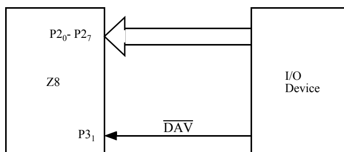
Figure 5-26. Input Strobed Handshake on Port 2
