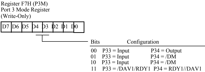
Figure 10-4. Port 3 Data Memory Operation
