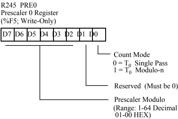
Figure 6-3. Prescaler 0 Register
