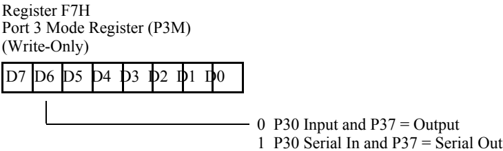
Figure 9-2. Port 3 Mode Register (P3M) and Bit-Rate Generation
