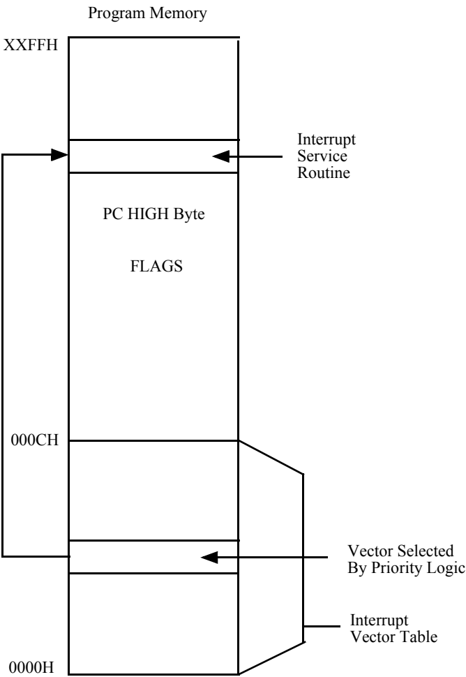
Figure 7-12. Interrupt Vectoring
