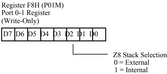
Figure 10-3. Z8 Stack Selection
