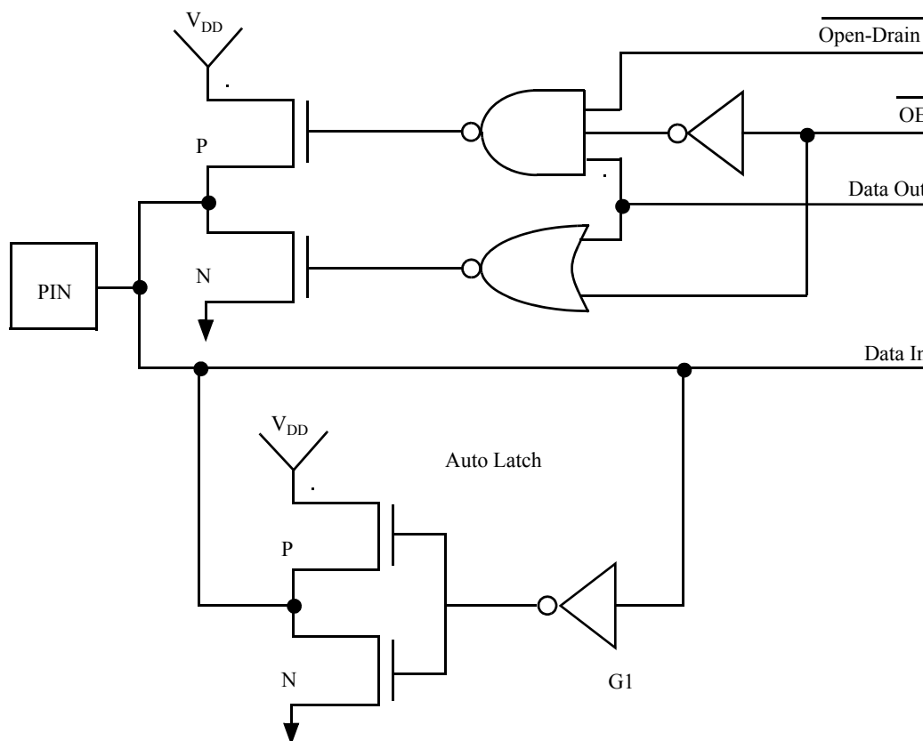
Figure 5-38. Simplified CMOS Z8 I/O Circuit
