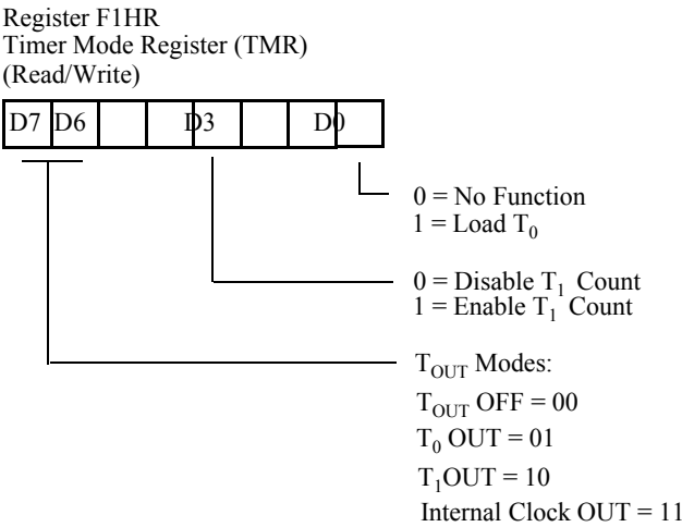
Figure 6-9. Timer Mode Register (T OUT Operation)
