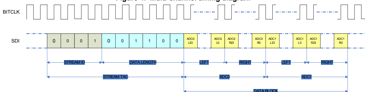
Figure 4. Multi-channel timing diagram
