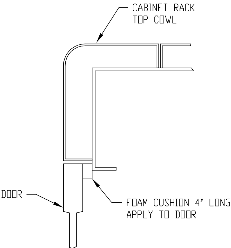
DETAIL "C"
